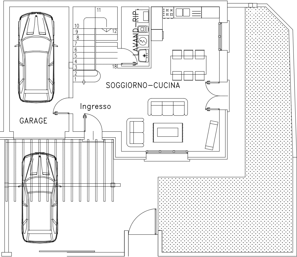
PIANO TERRA
